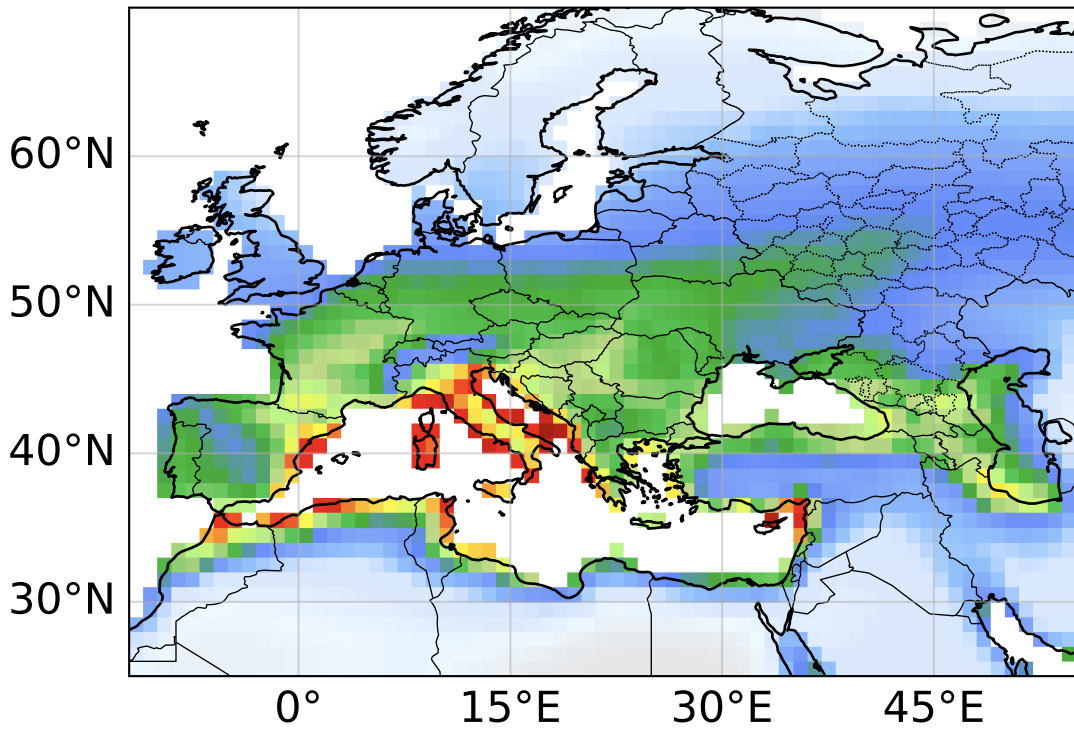
Mean
