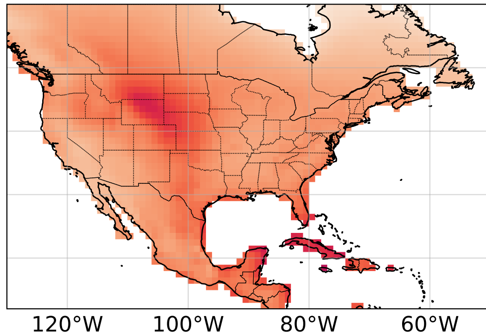
Standard deviation
