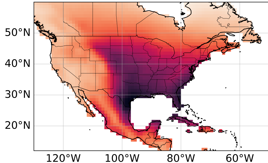
Mean
