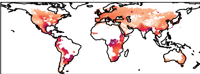
Barley (0.13)
