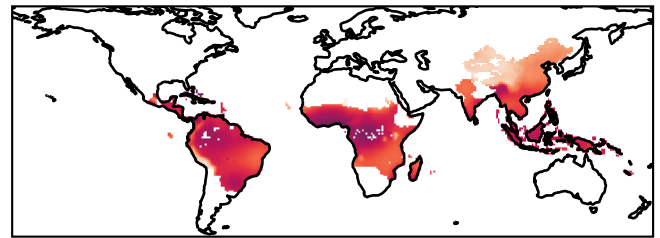
Others annual (0.21)
