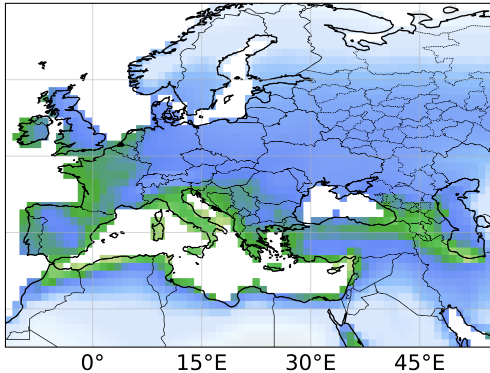
Standard deviation
