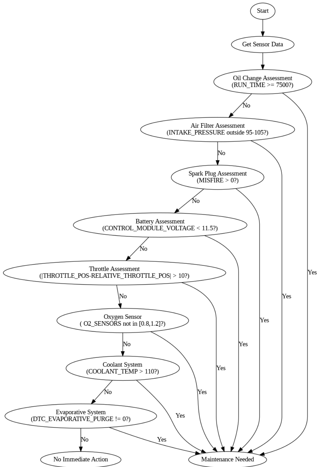
Figure 5.4: Comprehensive Flowchart of the Predictive Maintenance Router Diagnostic Process
