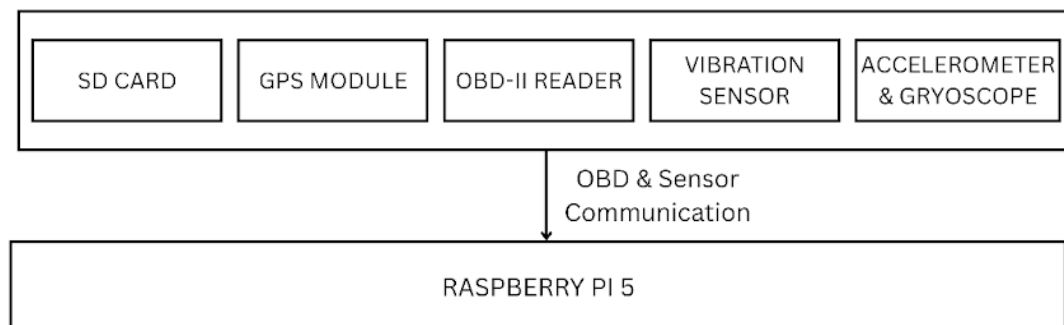
Figure 5.2: Flow Diagram Of Raspberry pi
