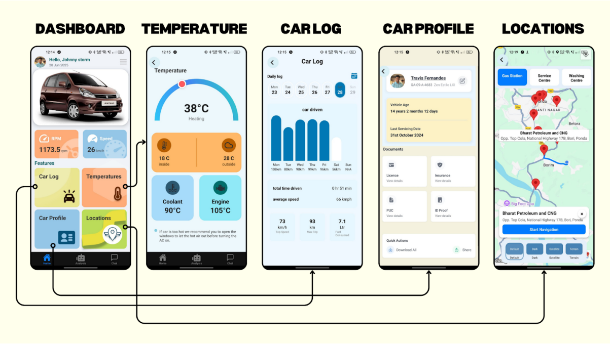
Figure 5.4: The dashboard includes direct navigation to four essential modules
