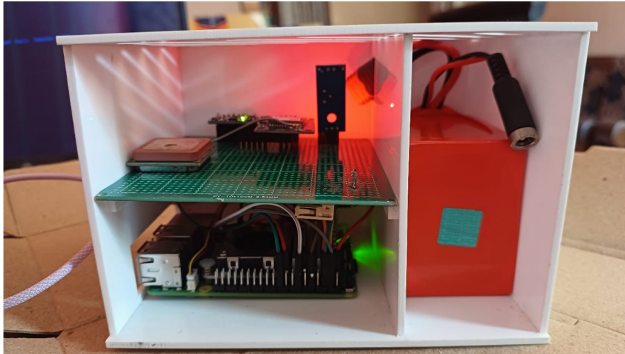
Figure 5.1: Automotive Diagnostic And Activity Monitoring (ADAM) BOX
