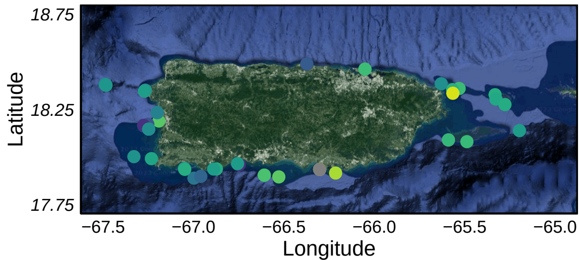
(e) Surface DO (mg/L)
