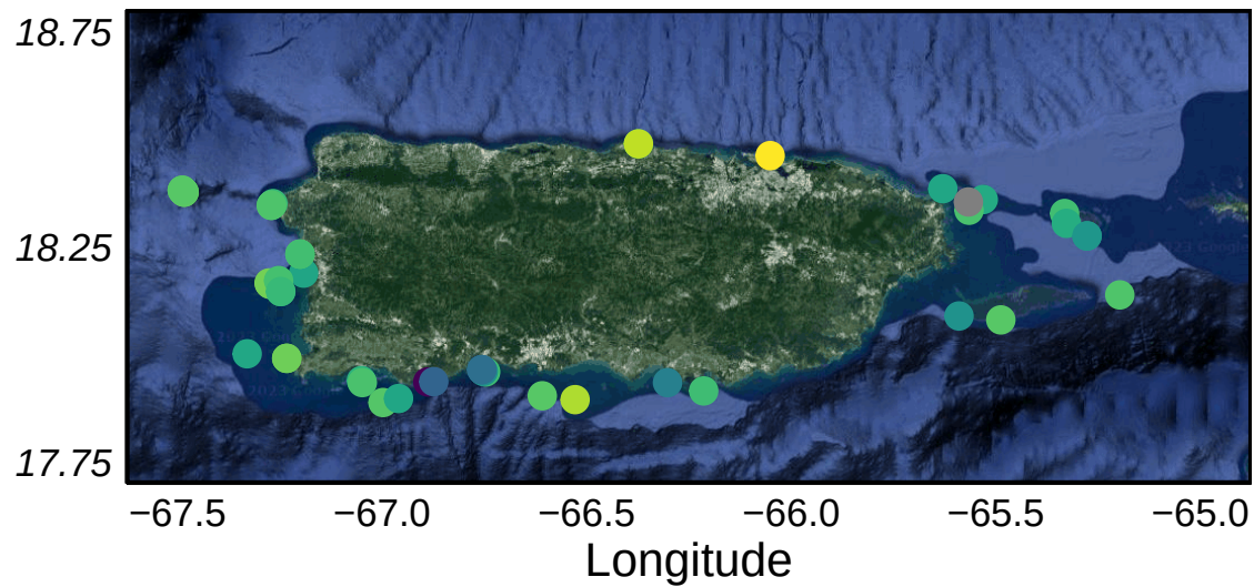
(f) Bottom DO (mg/L)
