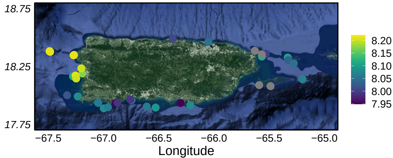
(h) Bottom pH
