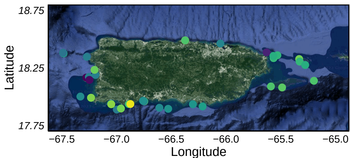
(a) Total Suspended Solids (mg/L)
