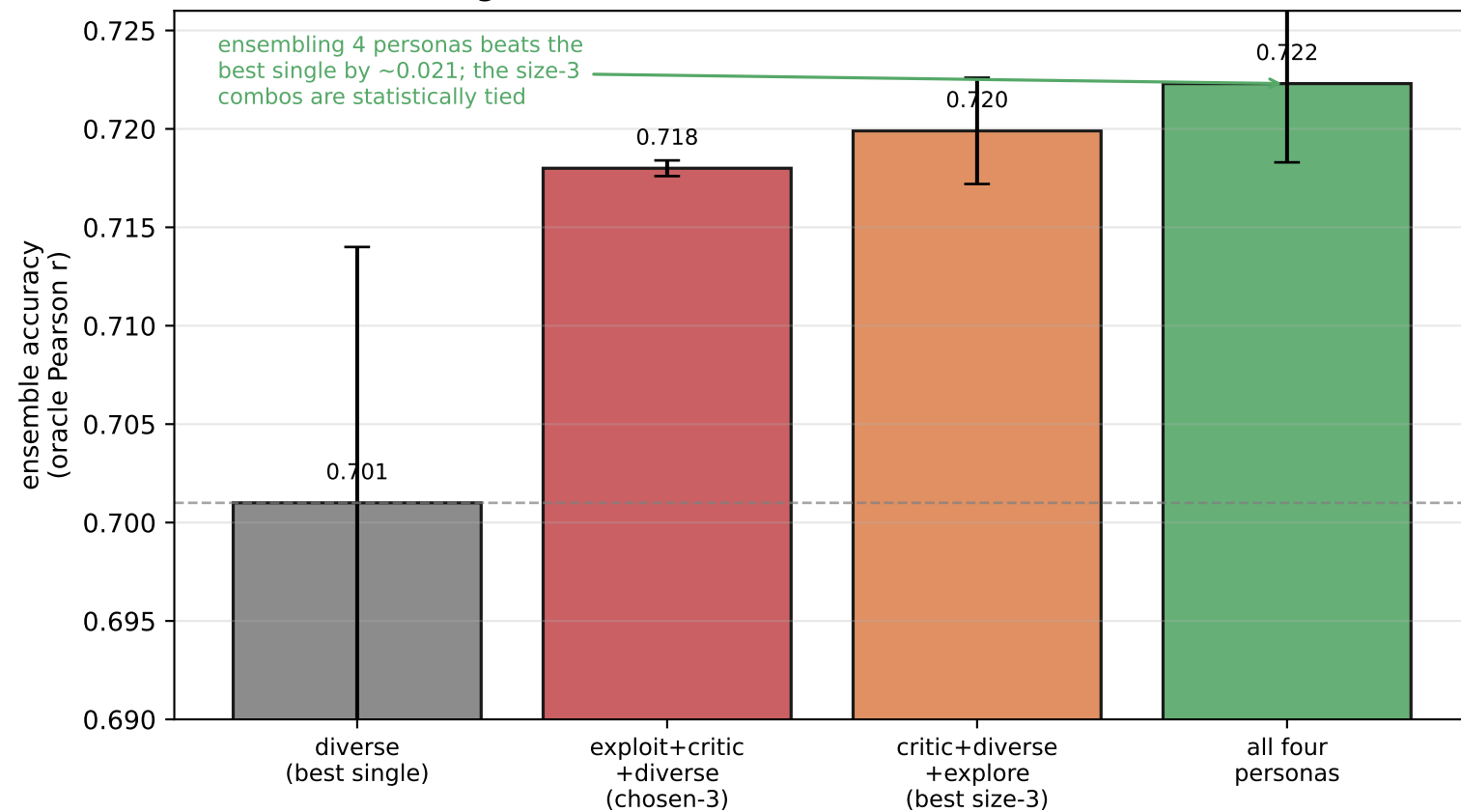
Phase 0: the LLM personas are COMPLEMENTARY (K562, genomic, D=30k, 3 seeds; ElasticNetCV ensemble)
