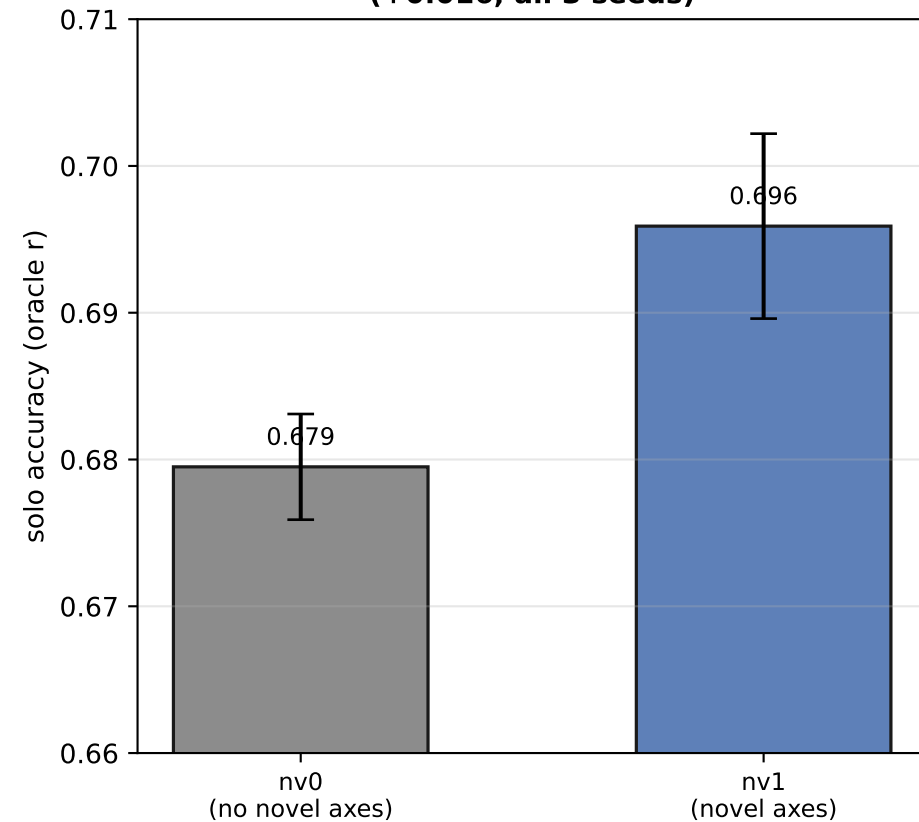
'Novel off-menu HP axes' help the diverse persona (+0.016, all 3 seeds)
