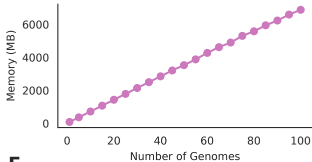
bronko call Memory Usage
