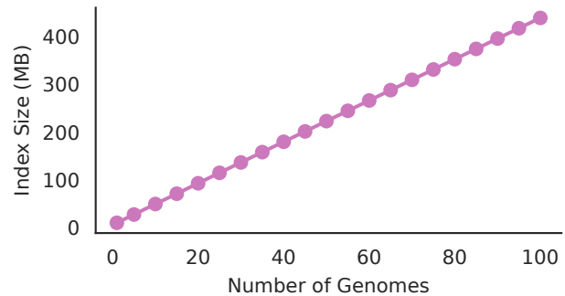
bronko Index Size
