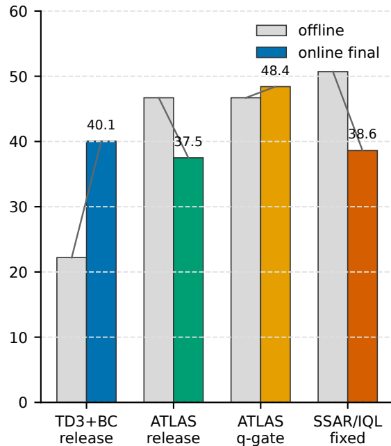
Offline endpoint vs online final
