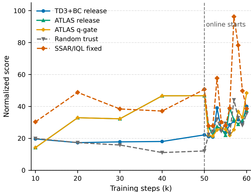
Eval20 O2O curves
