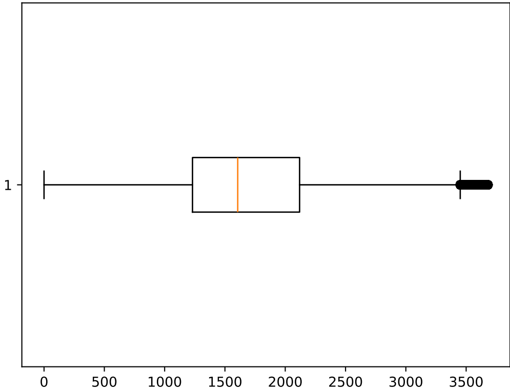
Distribution of LivingArea
