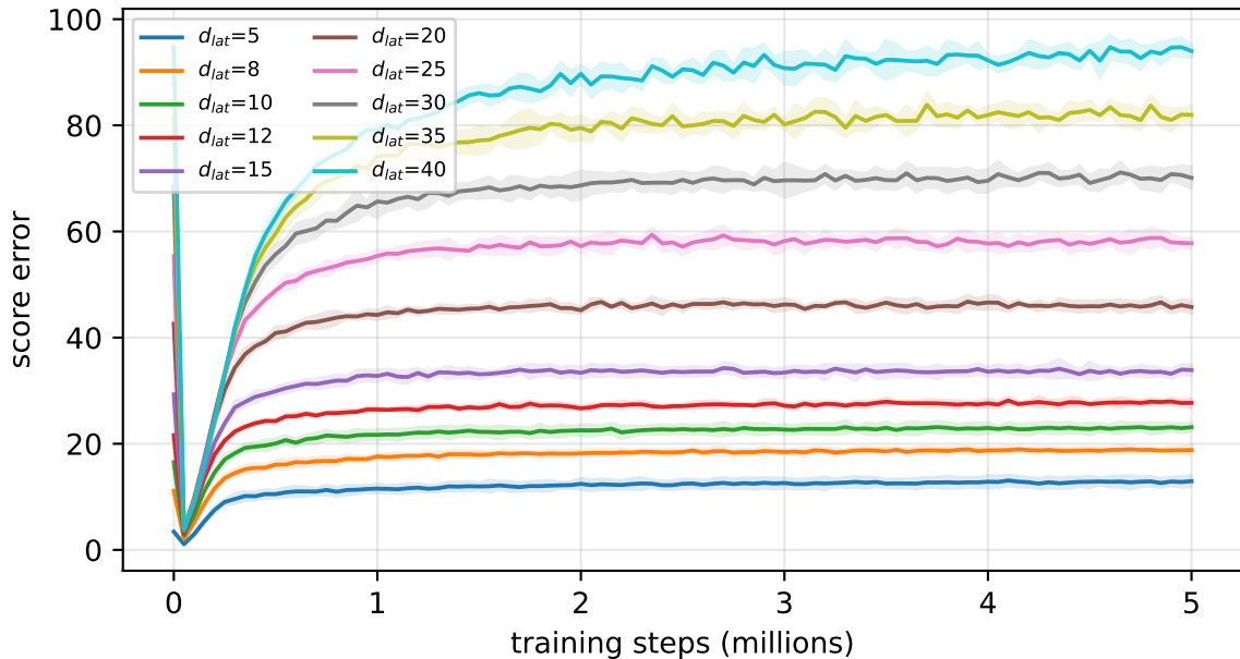
Corrected score error over training (t = 0.1), 5-seed mean with 95% CI
