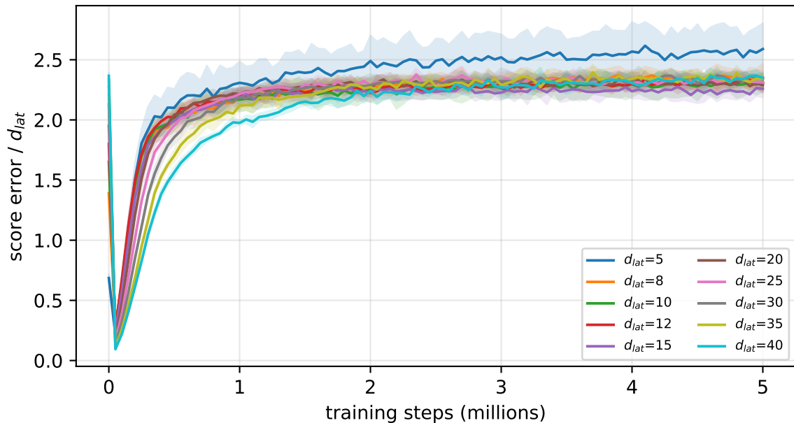
Corrected dimension-normalized score error over training ( t = 0.1 ), 5-seed mean with 95% CI
