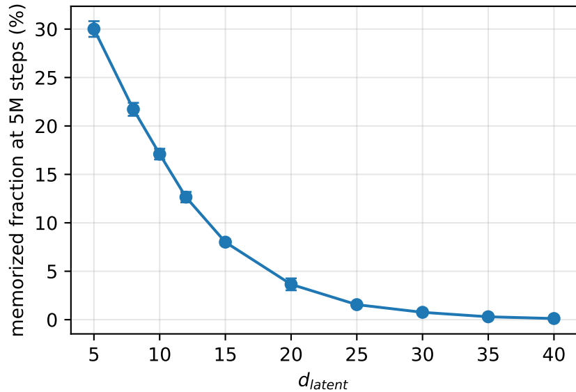
Fixed width: hidden = 256 (the caption's sweep)
