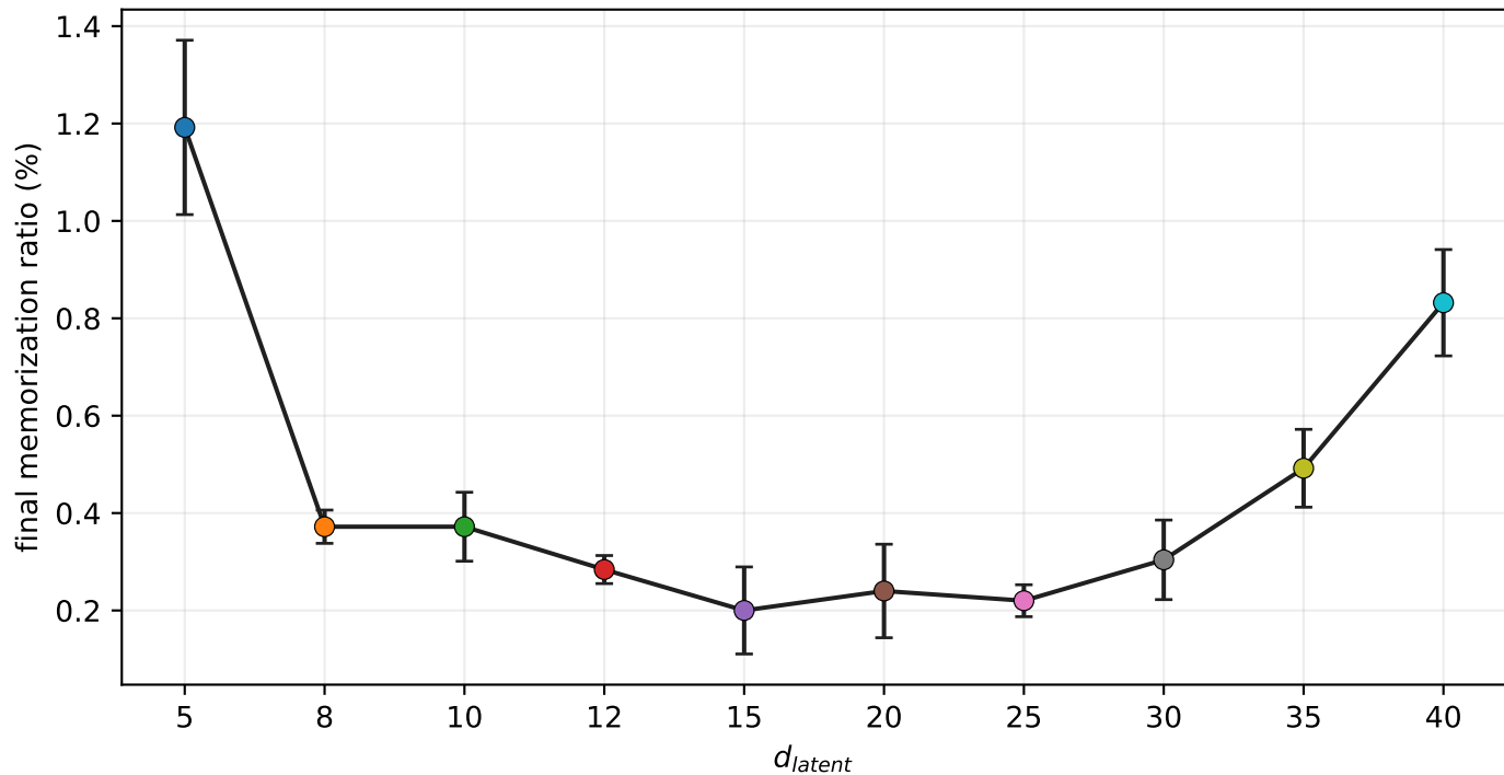
Final memorization ratio at 5M steps, 5-seed mean
