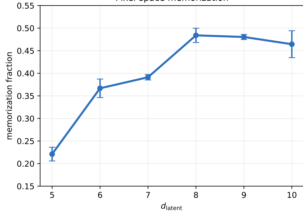
Pixel-space memorization
