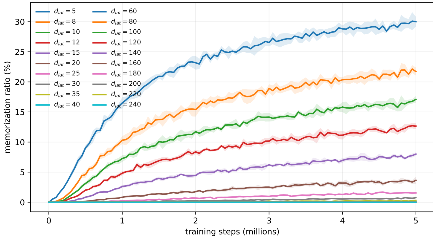
Memorization ratio over training, 5-seed mean with 95% CI
