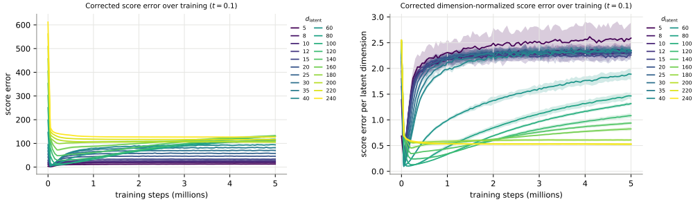
(a) Score error, all coordinates.
