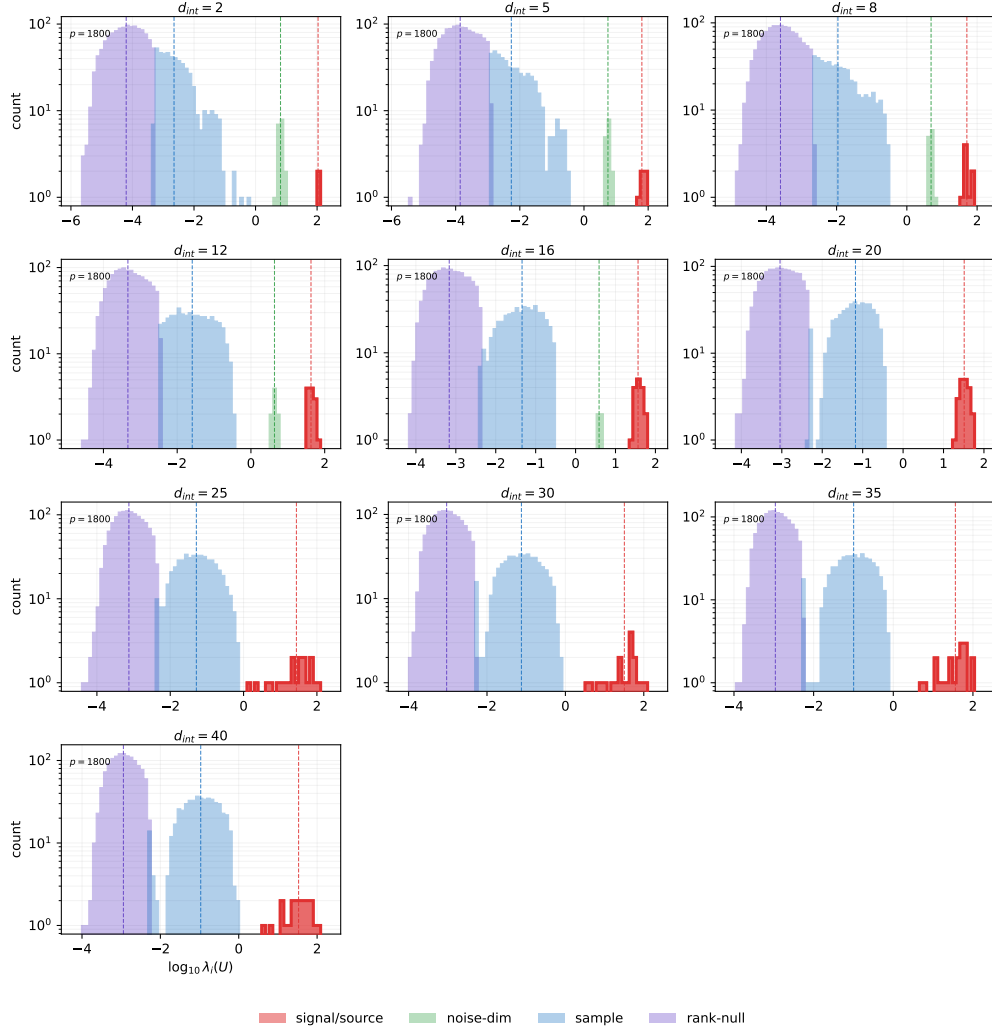
Figure 9: Experiment 2 RFNN source-dimensionality sweep with fixed width. For this control d_{latent} = 20 is fixed and d_{intrinsic} is swept as in the other Experiment 2 panels, while RFNN width is held fixed instead of growing with d_{latent} or d_{intrinsic} . For d_{intrinsic} > d_{latent} , the source structure is compressed into the fixed observed latent space, so the high- d_{intrinsic} regime should be read as an over-intrinsic stress test rather than a literal null-buffer regime. The fixed-width control makes the narrowing of the buffer visible without simultaneously changing RFNN capacity. The relevant regime is therefore decreasing until the exact boundary d_{intrinsic} = d_{latent} , followed by compressed over-intrinsic behavior rather than a new buffer. Colors are assigned by sorted eigenvalue-index blocks rather than fitted clusters: red denotes signal/source modes, green the observed latent-null/noise-dimension block, blue sample-specific modes, and purple rank-null modes. Dashed vertical lines mark the median log-eigenvalue of each colored block.
