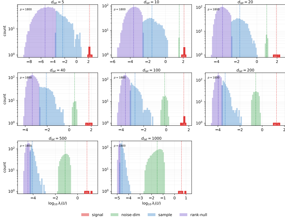
Figure 6: Experiment 1 RFNN four-bulk spectra for the latent-dimension sweep with fixed p = 1800 and fixed total null energy. The swept variable is still d_{\text{latent}} , but \sigma_{\perp}^2 is rescaled as E_{\text{null}}/(d_{\text{latent}} - d_{\text{intrinsic}}) so that the total null variance does not grow with latent dimension. This is the strictest control because increasing d_{\text{latent}} no longer increases either the number of random features or the total variance injected into null coordinates. The remaining spectral separation is therefore the cleanest evidence that the buffer arises from the distribution of modes across the latent space. The increasing regime is tied to the exact synthetic quantity d_{\text{latent}} - d_{\text{intrinsic}} , not to increasing RFNN width or total null energy. Colors are assigned by sorted eigenvalue-index blocks rather than fitted clusters: red denotes signal/source modes, green the observed latent-null/noise-dimension block, blue sample-specific modes, and purple rank-null modes. Dashed vertical lines mark the median log-eigenvalue of each colored block.
