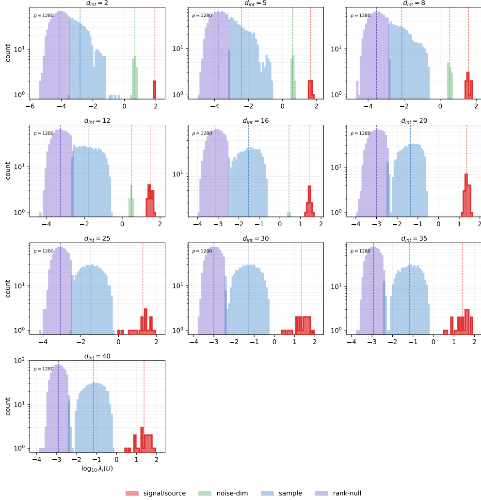
Figure 7: Experiment 2 RFNN source-dimensionality sweep with a fixed observed latent space under the p = 64d_{\text{latent}} width rule. The learned latent dimension is held fixed at d_{\text{latent}} = 20 , \sigma_{\text{signal}} = 1.0 , \sigma_{\perp} = 0.5 , and GMM center scale 3.0, while the intrinsic dimension of the source distribution sweeps d_{\text{intrinsic}} \in \{2, 5, 8, 12, 16, 20, 25, 30, 35, 40\} . When d_{\text{intrinsic}} < d_{\text{latent}} , the remaining observed coordinates form a genuine null buffer; as d_{\text{intrinsic}} approaches d_{\text{latent}} , that buffer shrinks and the signal and sample regions become less separated. Because d_{\text{latent}} = 20 is fixed and known, this is the exact decreasing-buffer regime: the green block shrinks as d_{\text{latent}} - d_{\text{intrinsic}} and disappears at d_{\text{intrinsic}} = d_{\text{latent}} . Colors are assigned by sorted eigenvalue-index blocks rather than fitted clusters: red denotes signal/source modes, green the observed latent-null/noise-dimension block, blue sample-specific modes, and purple rank-null modes. Dashed vertical lines mark the median log-eigenvalue of each colored block.
