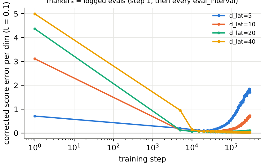
exp2_h256_sn001_300k: corrected error vs step (mean \pm sd over seeds) markers = logged evals (step 1, then every eval_interval)
