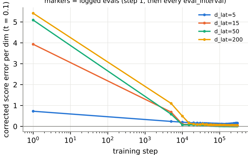
exp2_scaled_sn001_300k: corrected error vs step (mean \pm sd over seeds) markers = logged evals (step 1, then every eval_interval)
