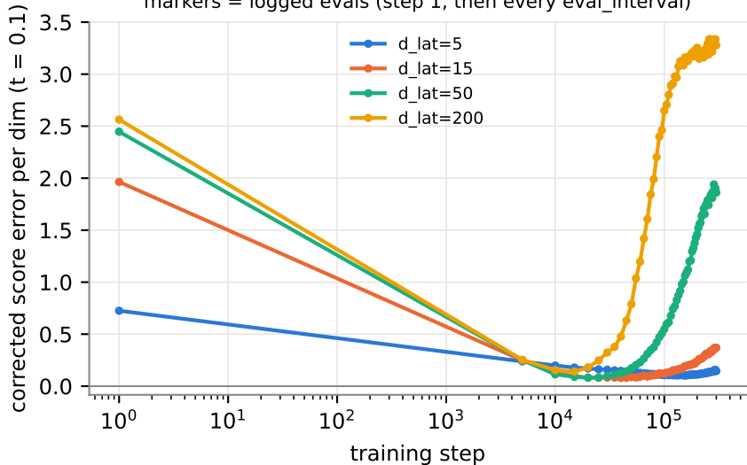
exp2_scaled_sn05_300k: corrected error vs step (mean \pm sd over seeds) markers = logged evals (step 1, then every eval_interval)
