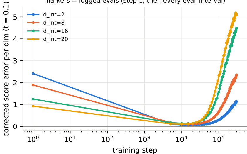
exp3_dint_h256_sn05_300k: corrected error vs step (mean \pm sd over seeds) markers = logged evals (step 1, then every eval_interval)
