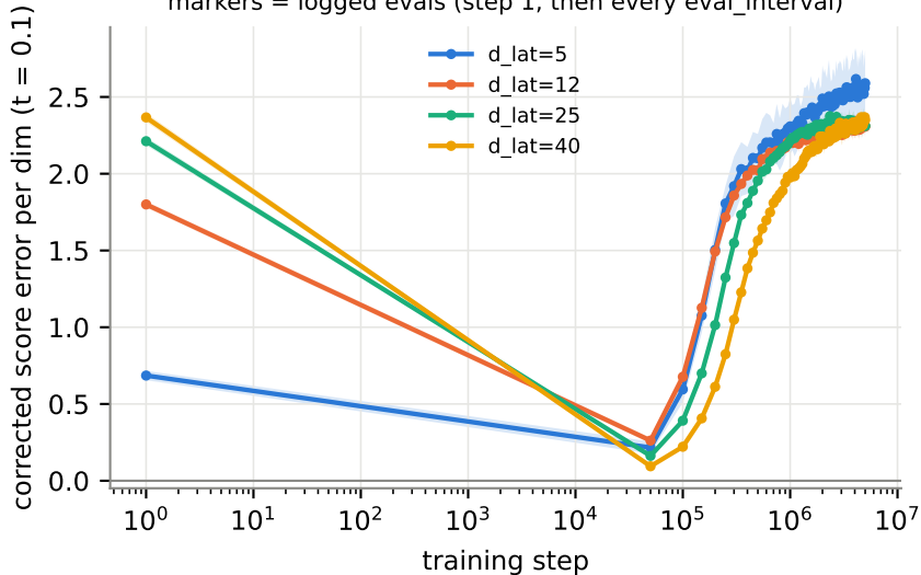
paper_h256_5seed_sn05_5M: corrected error vs step (mean \pm sd over seeds) markers = logged evals (step 1, then every eval_interval)
