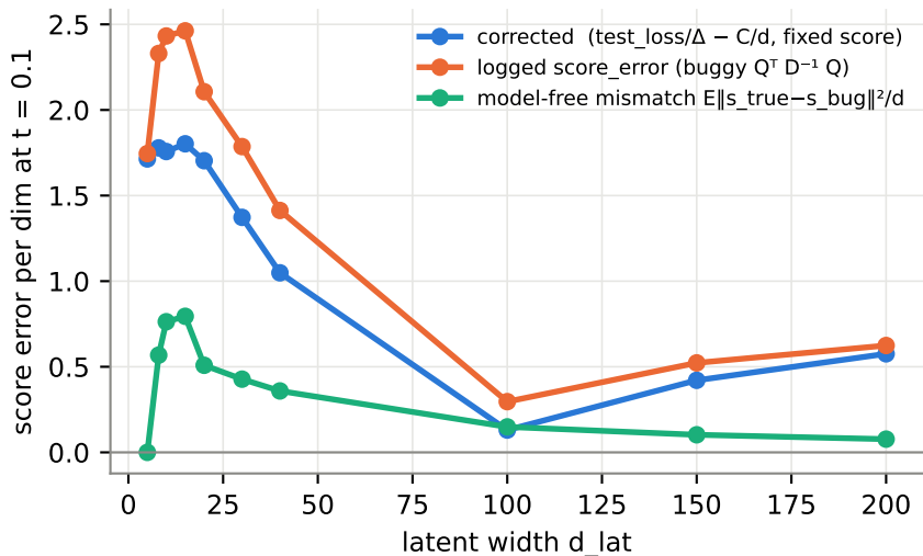
exp2_h256_sn05_300k final step 300000, 1 seed(s), band = \pm 1 sd over seeds
