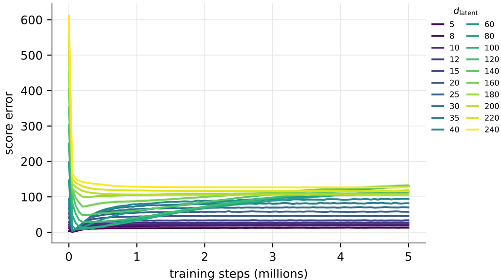
Corrected score error over training ( t = 0.1 )
