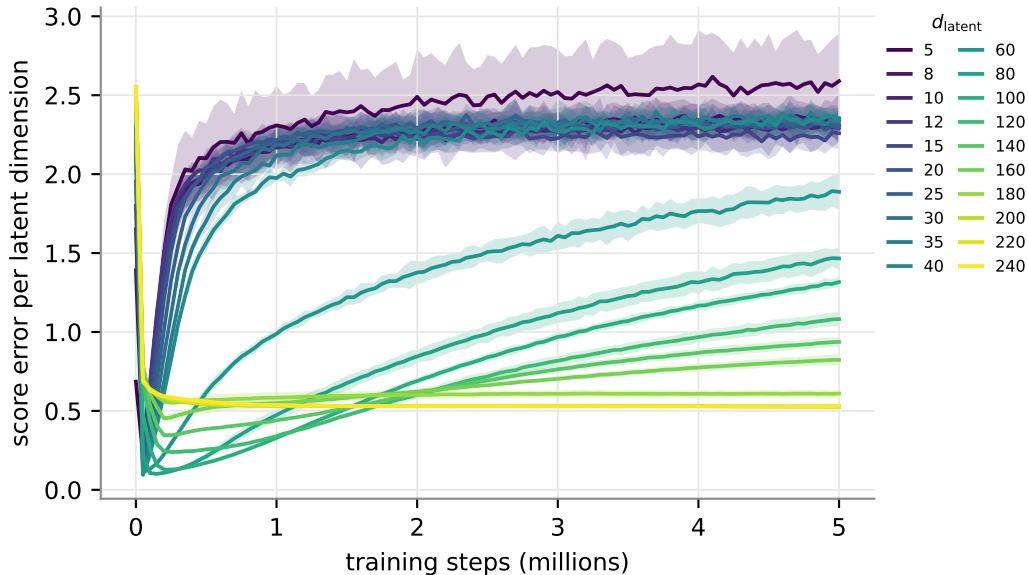
Corrected dimension-normalized score error over training ( t = 0.1 )
