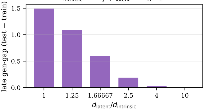
MLP d_{\text{intrinsic}} sweep ( d_{\text{latent}} = 20 ), \sigma_{\perp} = 0.01
