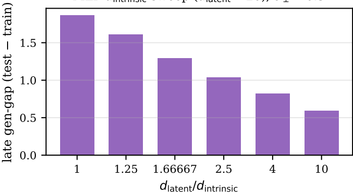
MLP d_{\text{intrinsic}} sweep ( d_{\text{latent}} = 20 ), \sigma_{\perp} = 0.5
