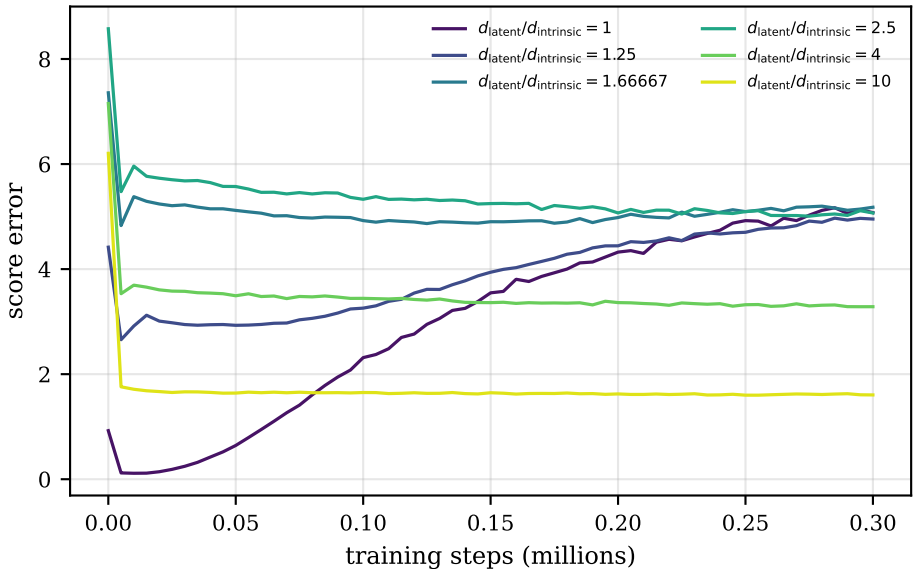
MLP d_{\text{intrinsic}} sweep ( d_{\text{latent}} = 20 ), \sigma_{\perp} = 0.01
