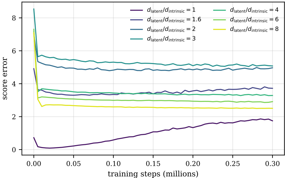
MLP, \sigma_{\perp} = 0.01
