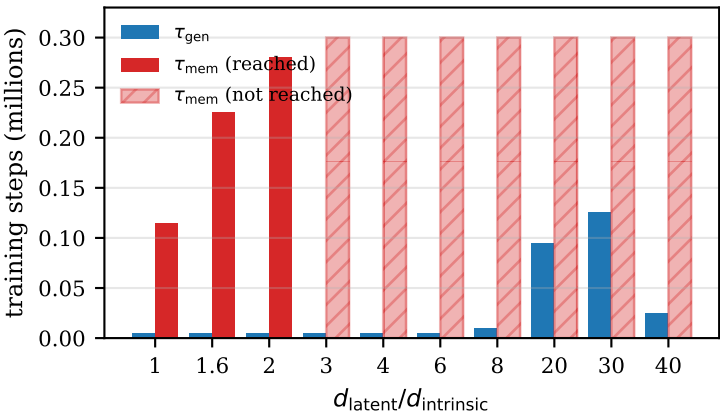
MLP, \sigma_{\perp} = 0.5
