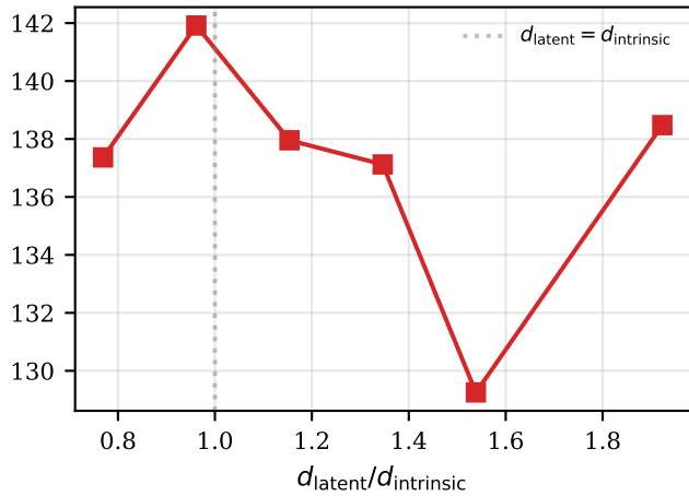
CelebA ( d_{\text{intrinsic}} \approx 26 ), n = 1000
