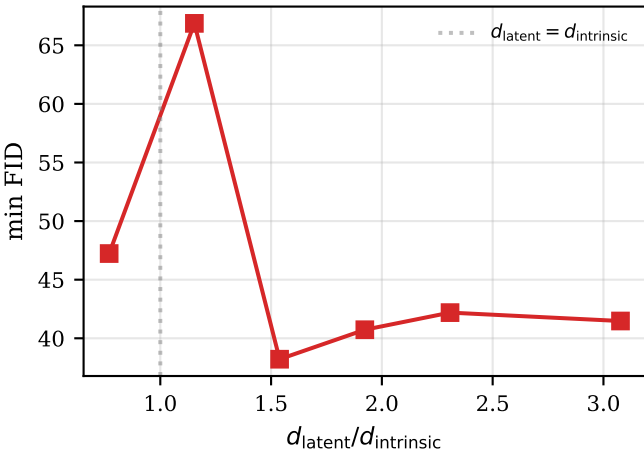
MNIST ( d_{\text{intrinsic}} \approx 13 ), n = 1000
