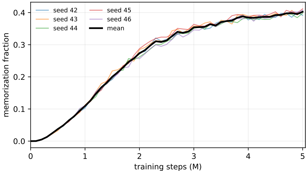
CIFAR-10 d=80
