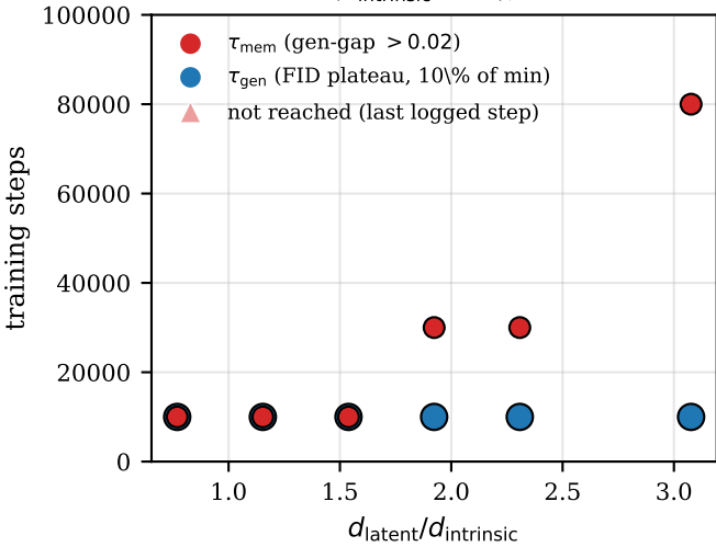
MNIST ( d_{\text{intrinsic}} \approx 13 ), n = 1000
