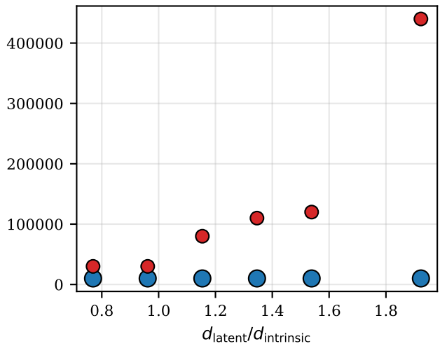
CelebA ( d_{\text{intrinsic}} \approx 26 ), n = 1000
