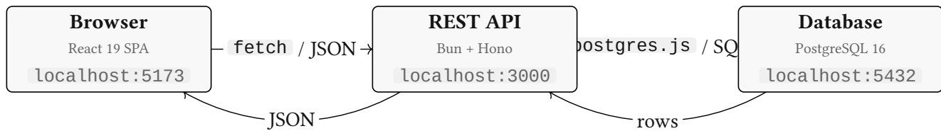
Figure 1: Three-tier architecture — the React SPA issues fetch calls to the Hono REST API, which sends parameterized SQL to PostgreSQL via the postgres.js driver.
