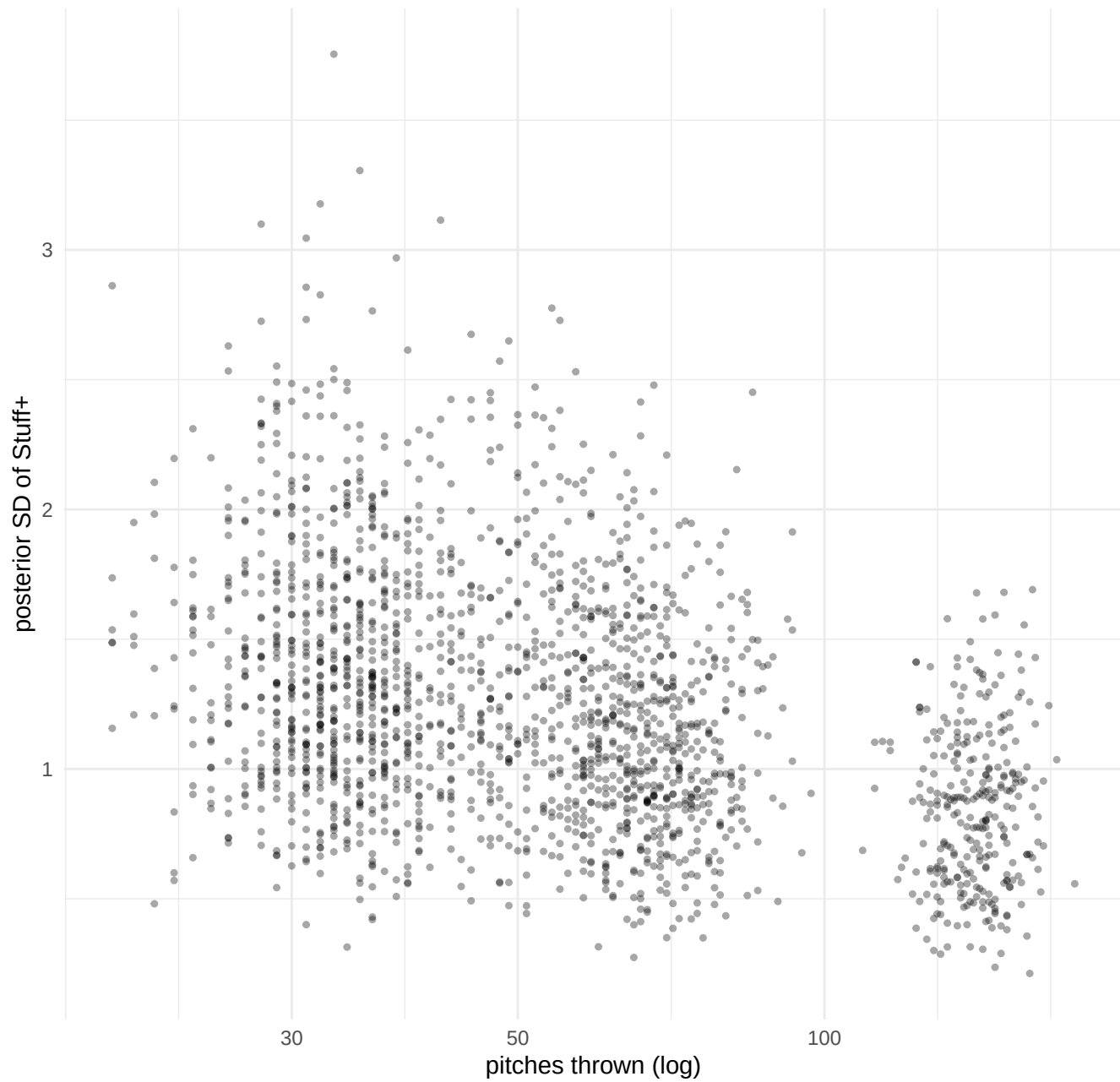
Uncertainty shrinks with sample size
