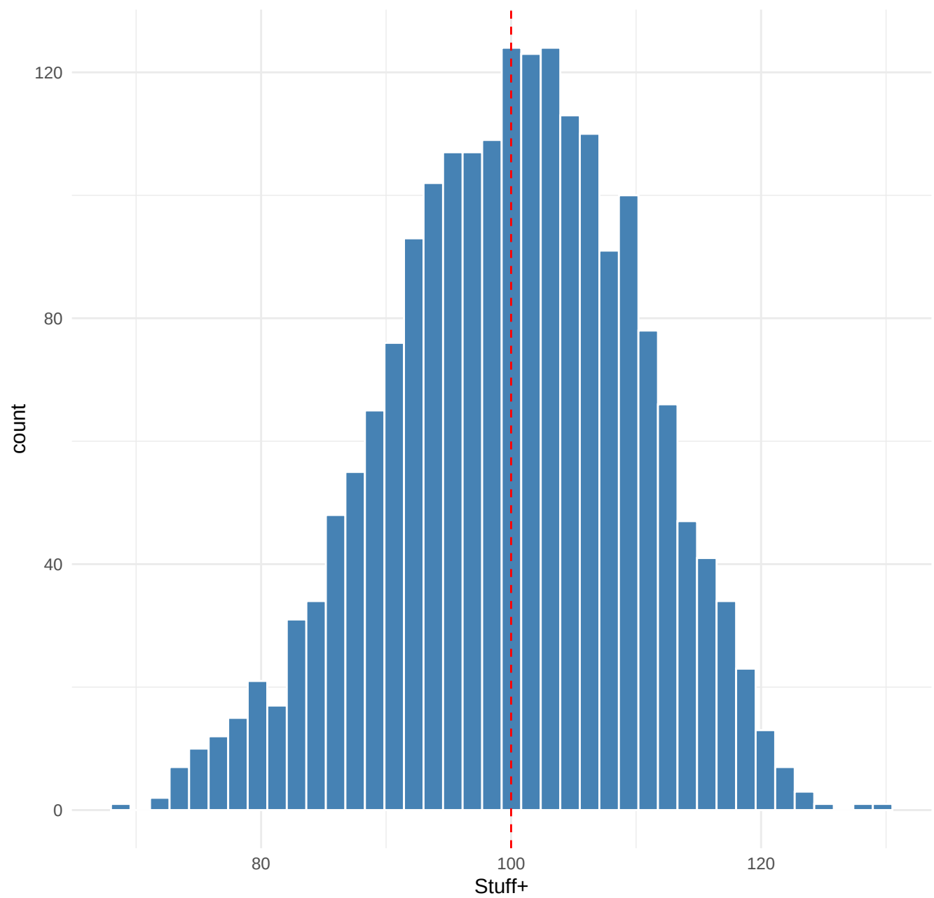
Stuff+ distribution (M1)
