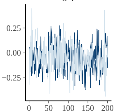
b_avg_pfx_z
