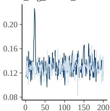
o_avg_release_extensor
