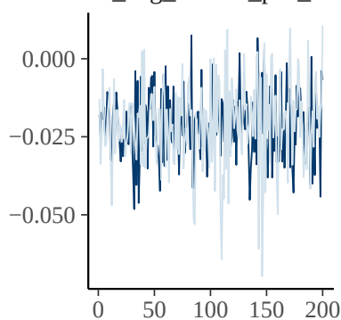
b_avg_release_pos_z
