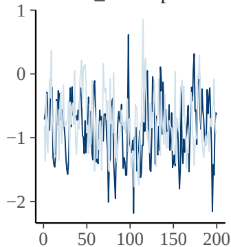
b_Intercept
