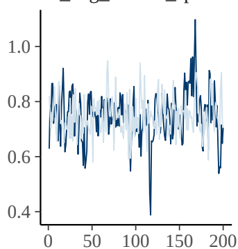
b_avg_release_speed
