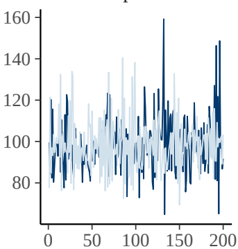
phi
