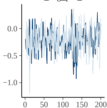
b_avg_pfx_x
