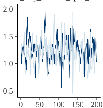
o_avg_release_spin_rate
