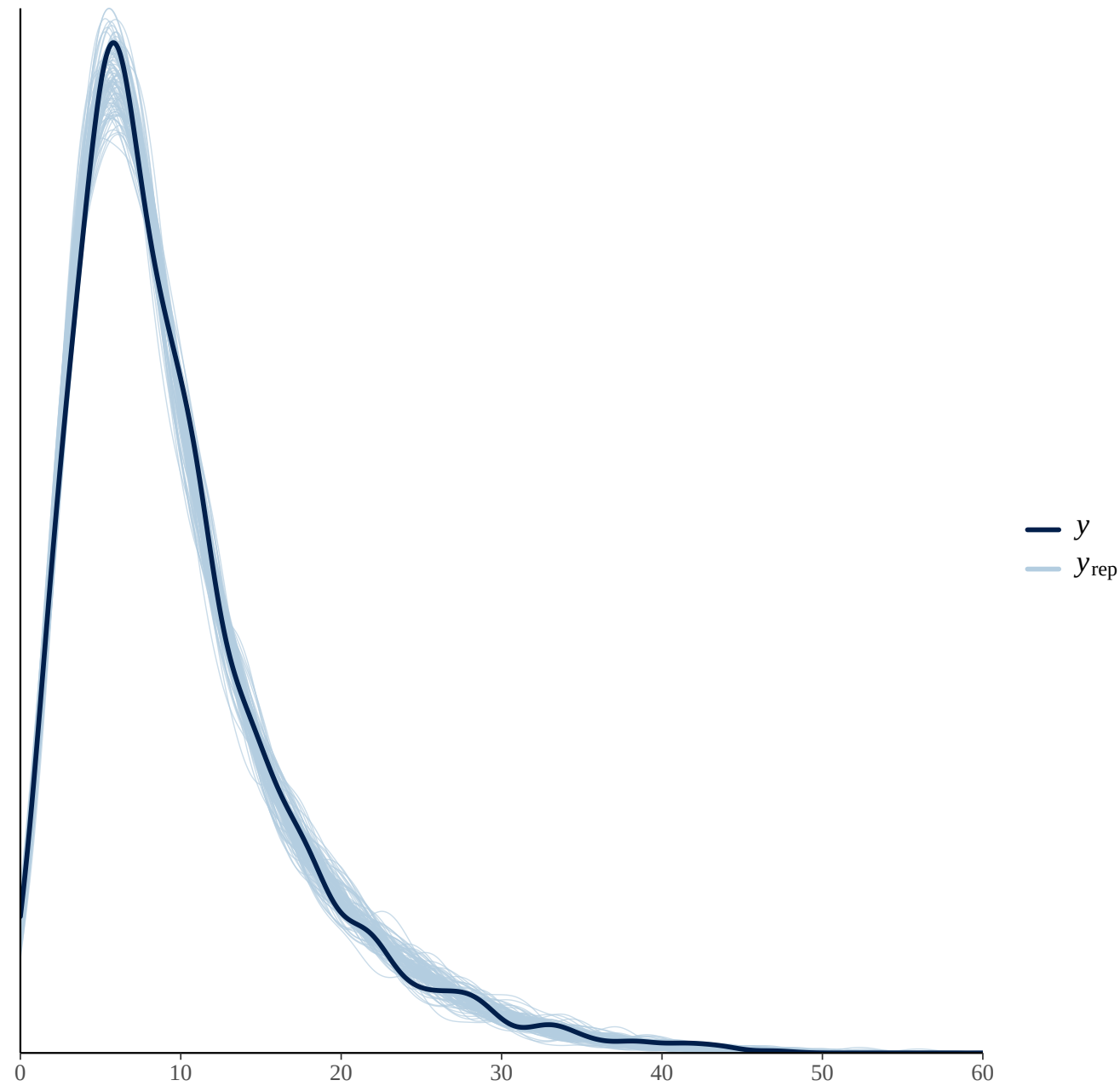
PPC ... whiff counts, M1
