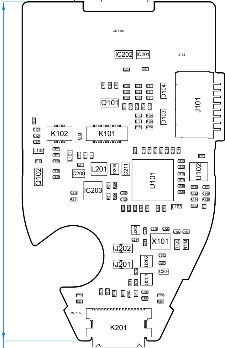
View from Top side (Scale 2.5:1)
