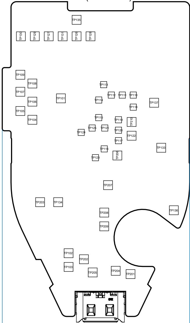
View from Bottom side (Scale 2.5:1)
