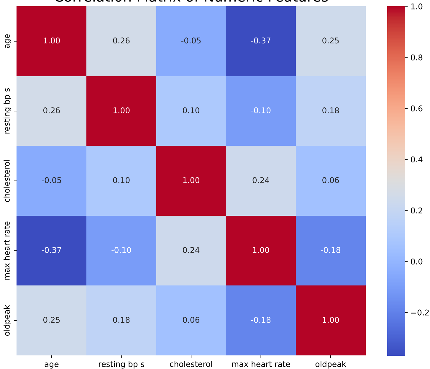
Correlation Matrix of Numeric Features
