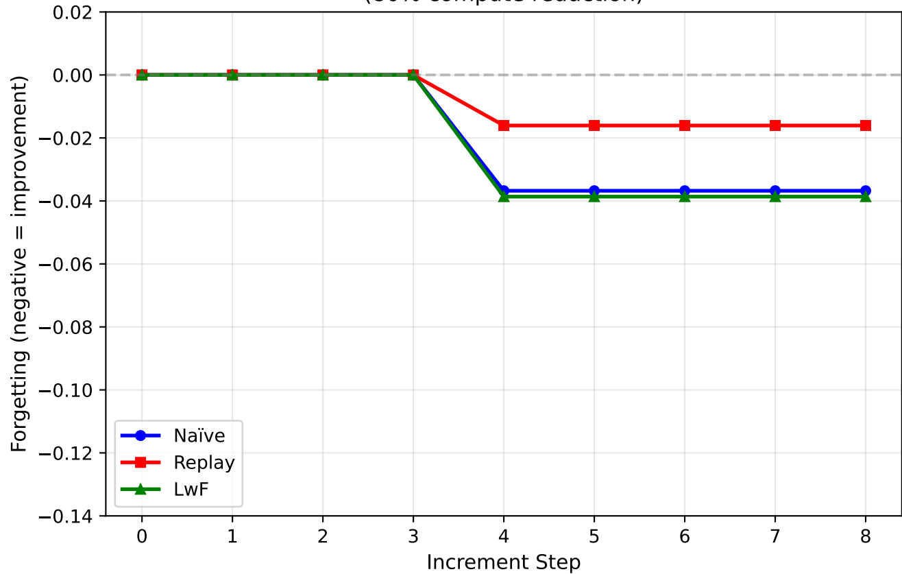
(B) K=5: Retrain every 5th increment (80% compute reduction)
