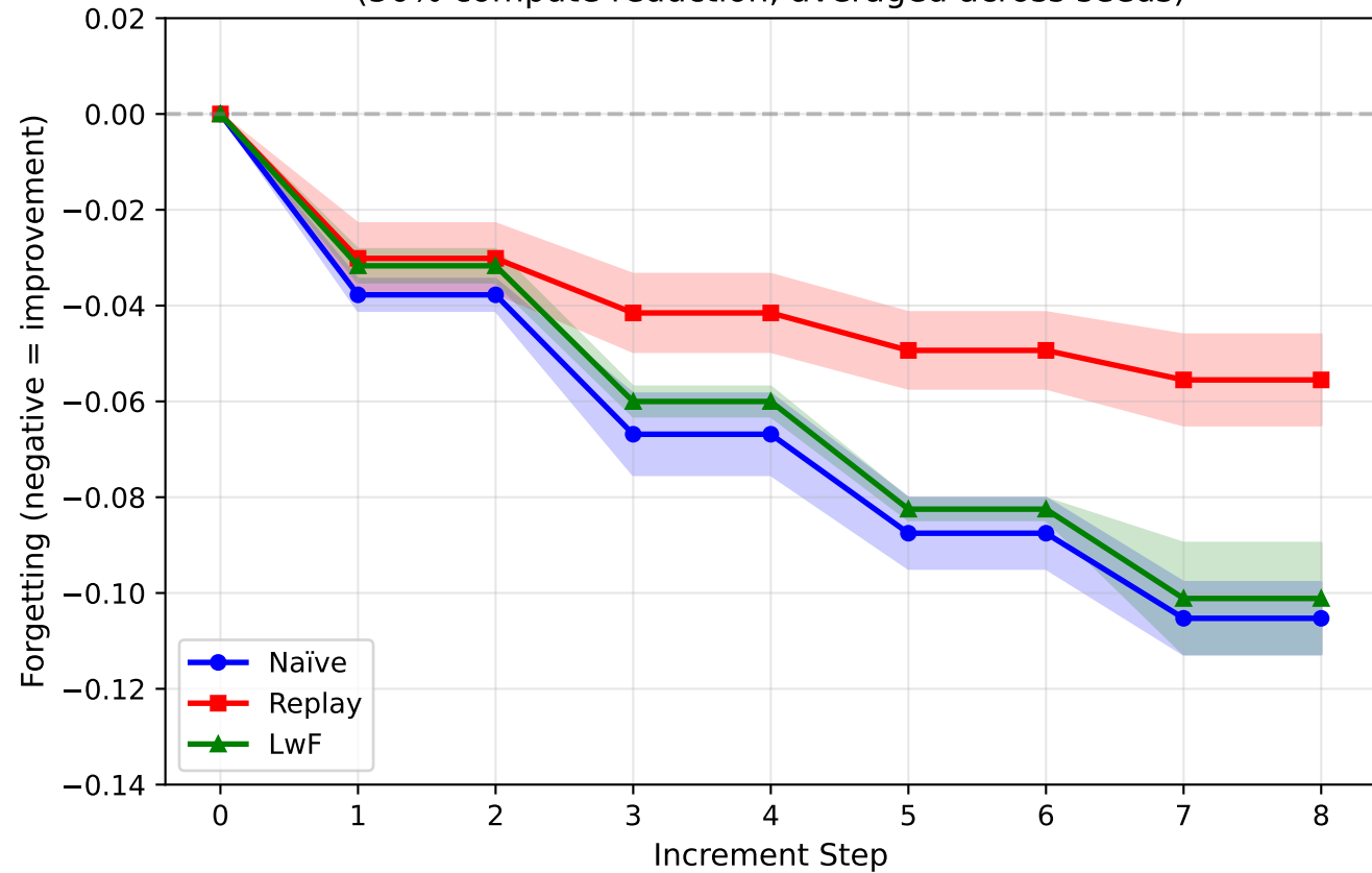
(A) K=2: Retrain every 2nd increment (50% compute reduction, averaged across seeds)
