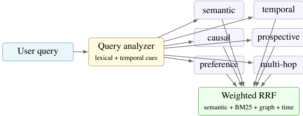
Figure 3.7: Adaptive Query Routing
