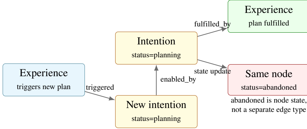
Figure 4.4: Intention Lifecycle
