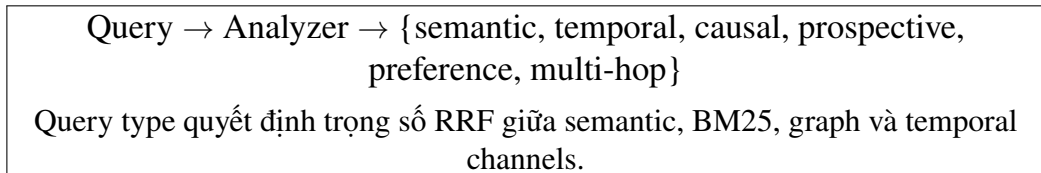
Figure 3.7: Adaptive Query Routing
