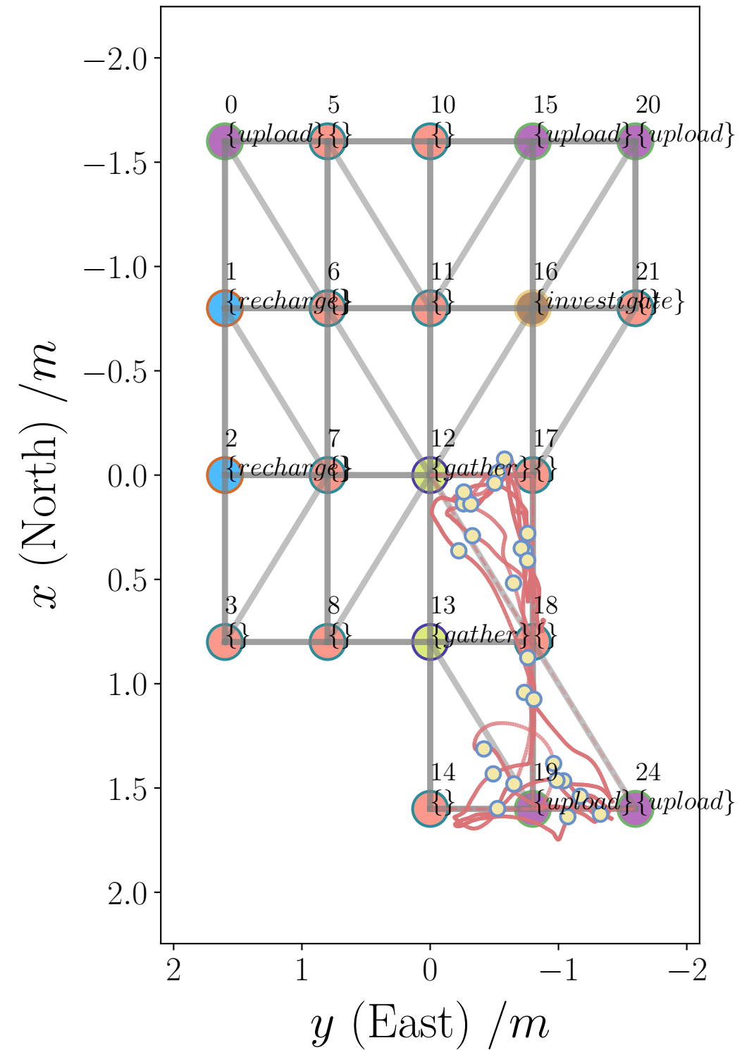
Horizontal Projection
