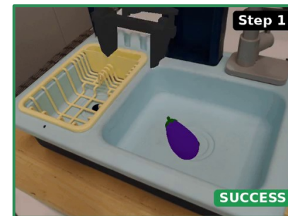
Foveation 20%
