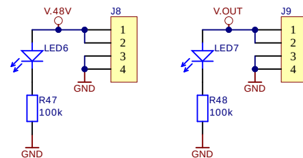
Power ports
