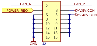
Deck slot connector
