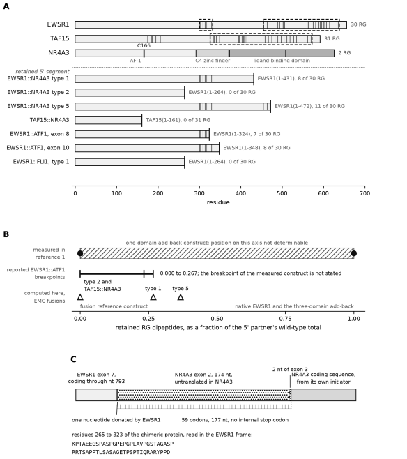
Figure 1. Reported EMC junctions on the retained-RG axis, and the type-2 seam. Three panels, drawn by emc_fusion_frame_figure.py and committed as emc-fusion-frame-fig1.png and emc-fusion-frame-fig1.pdf.
