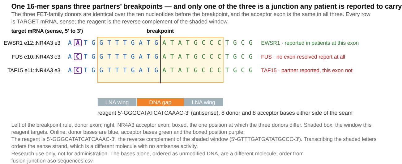
Figure 1. One 16-mer spans three partners' breakpoints, and only one of the three is a junction any patient is reported to carry. The junction windows of EWSR1 exon 12, TAF15 exon 11 and FUS exon 10 joined to NR4A3 exon 3, aligned at the breakpoint, each row carrying its own reporting status.
