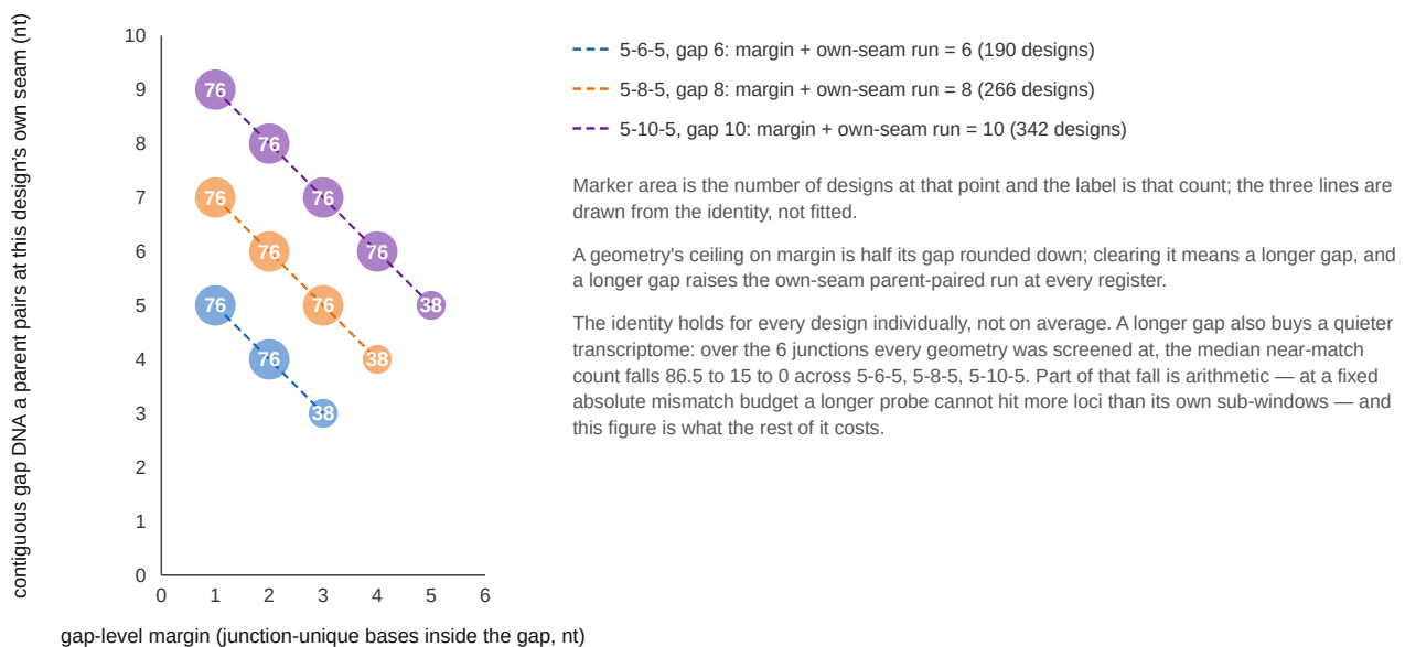
Figure 3. The margin a longer catalytic gap wins is the gap DNA a parent pairs at the design's own seam. (A) The best-margin design at EWSR1 exon 12 joined to NR4A3 exon 3, drawn at 5-6-5, 5-8-5 and 5-10-5 with the wings held at five nucleotides. Every base inside the catalytic gap comes from the donor exon or from the acceptor exon, so the junction-unique bases on the shorter side and the bases one wild-type parent pairs on the longer side tile the gap and sum to it. (B) Every fusion-specific design in all three geometries, 798 over 38 junctions, plotted as gap-level margin (abscissa) against the contiguous run of gap DNA one of the design's OWN two parents pairs at its seam (ordinate). That is not the quantity the markers and the do-not-order verdicts are set on. Those come from a SEARCH over all six mature parent transcripts, and the two separate: for the molecule drawn in (A) this figure draws 3 nucleotides where Tables 2, 3, 5 and 7 print an 8 bp duplex against wild-type TFG . The two also move in opposite directions across the geometries — the searched duplex FALLS (181 of 190, then 130 of 266, then 87 of 342 pair a parent at any length) and is flat at the ten-base-pair criterion (87, 88, 87), while the quantity drawn here RISES (76 of 190, 228 of 266, 342 of 342). A longer gap concedes seam-level parent DNA; it does not concede more of the liability this paper condemns. In (A) red marks the gap bases contributed by the donor exon, green those contributed by NR4A3 , and pale grey the LNA wings, which are not cleaved; the shorter of the two coloured runs is the margin and the longer is what a wild-type parent can pair, so which colour is which depends on the register — the junction drawn here divides its gap evenly in all three geometries, and 76 of the 190 designs at 5-6-5 have the longer run on the donor side; in (B) the three geometries are blue (5-6-5), orange (5-8-5) and purple (5-10-5). Both panels repeat these keys beside the drawing. Marker area is the number of designs at that point and the label is that count; the three lines are drawn from the identity, not fitted, and it holds for each design individually rather than on average. Within one geometry the two move inversely along a line of slope -1, and both axes are drawn at the same scale (32 px per nucleotide) so that slope is true as plotted rather than only in the units; a geometry's ceiling on margin is half its gap rounded down, and clearing it means a longer gap and a higher parent-paired run at every register (§2.9, Table 7).
