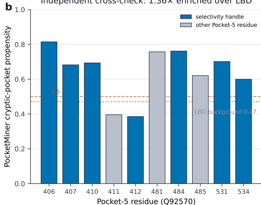
Independent cross-check: 1.36 \times enriched over LBD
