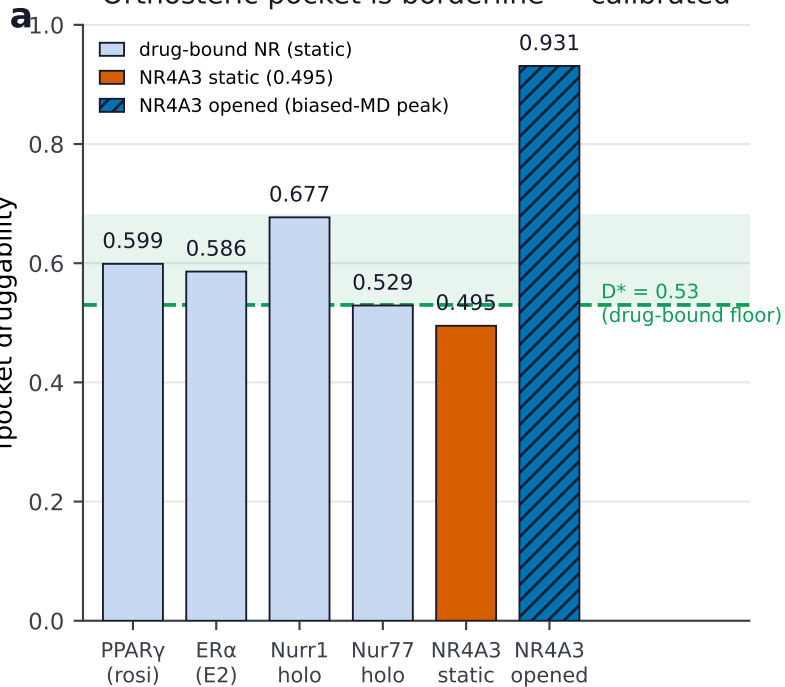
Orthosteric pocket is borderline — calibrated
